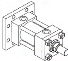
Square Cap Flange Style MF6
