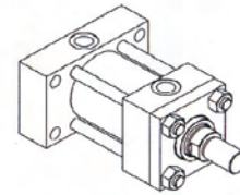
Rectangular Cap Mount Style ME6
