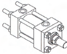
Tie Rod Extended Cap Style MX2
