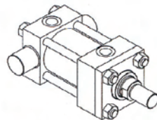
Cap Trunnion Style MT2
